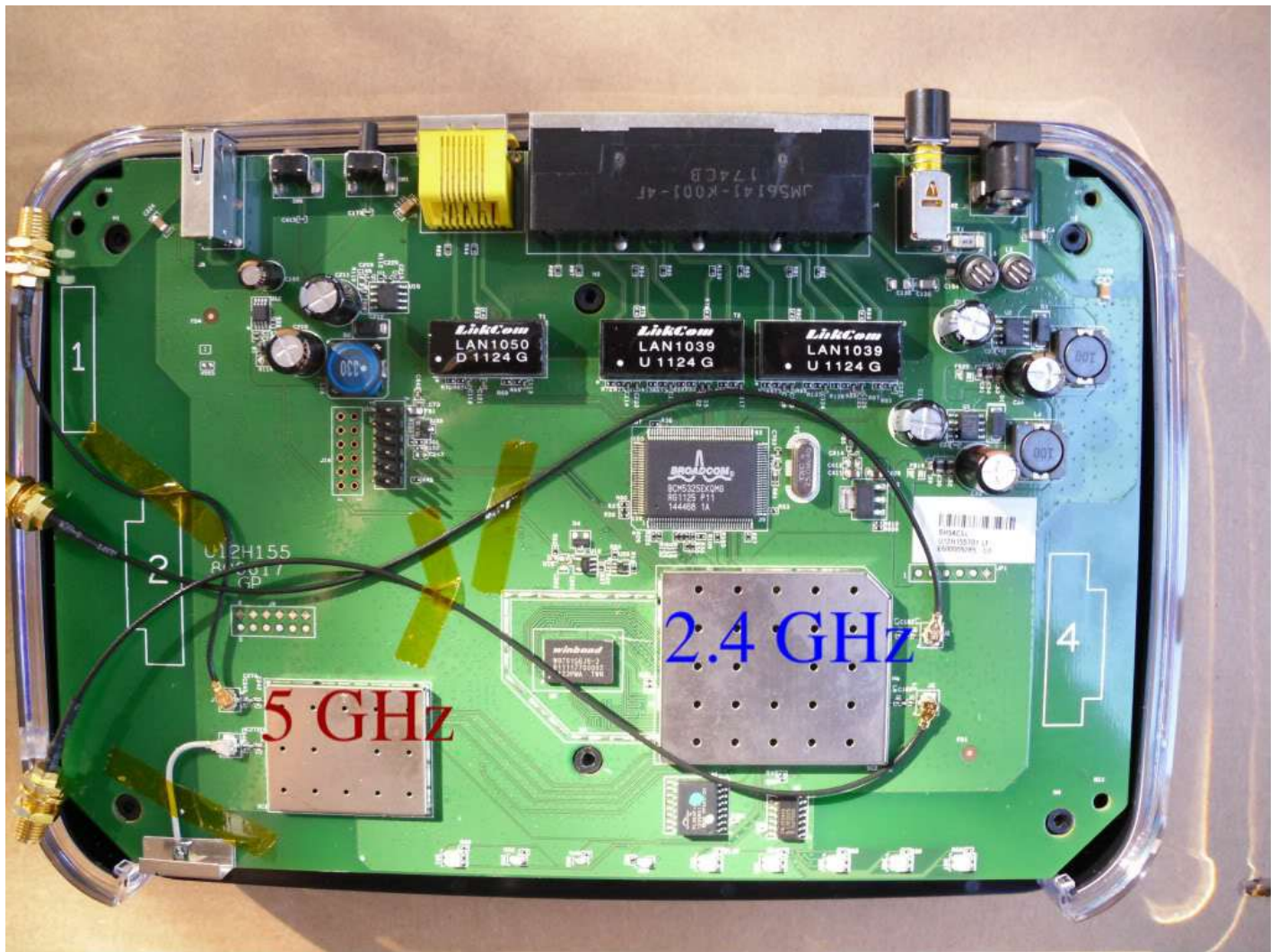
After Modification V1 (you can choose which antenna to mod depending on your preference)
