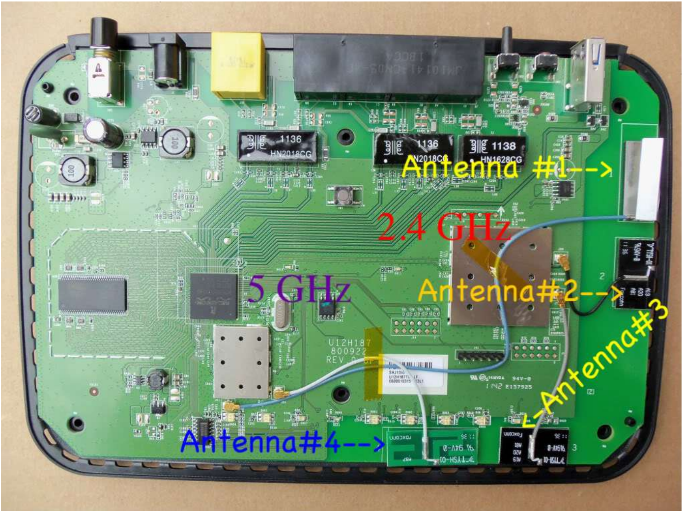
Before the mod Version 2
