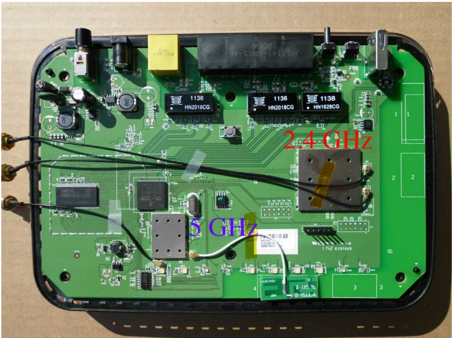
After the modification Version 2
